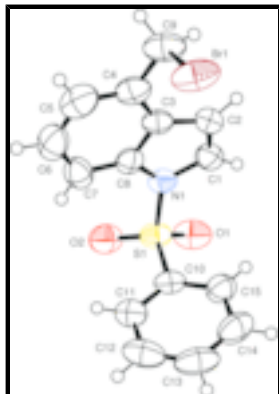
Fig. 1. The molecular structure of (I) showing the atomic labels and 50% probability displacement ellipsoids for non-H atoms. Only major parts of the disordered atoms are drawn.
